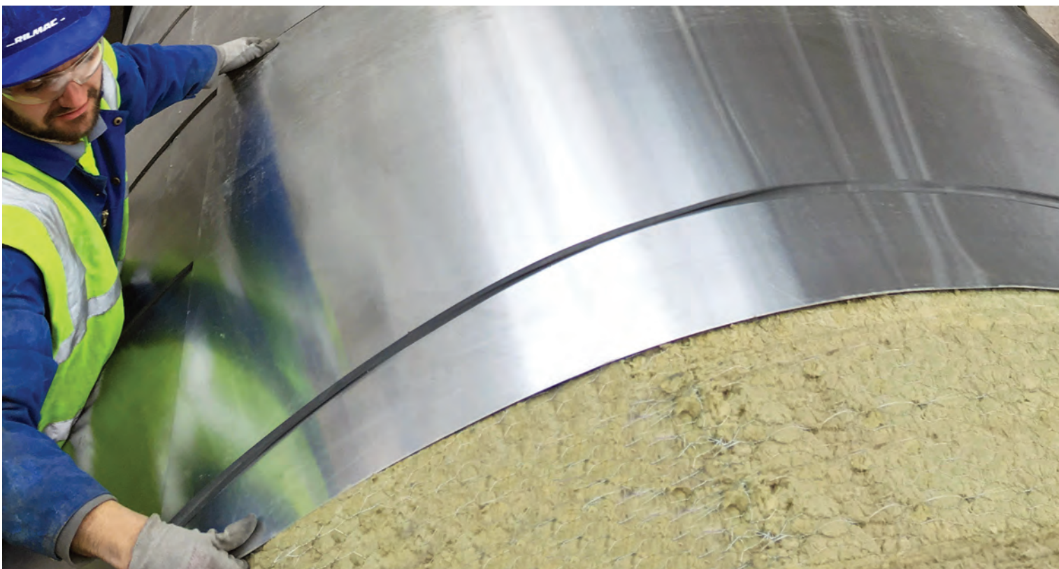
External insulation at cement works
